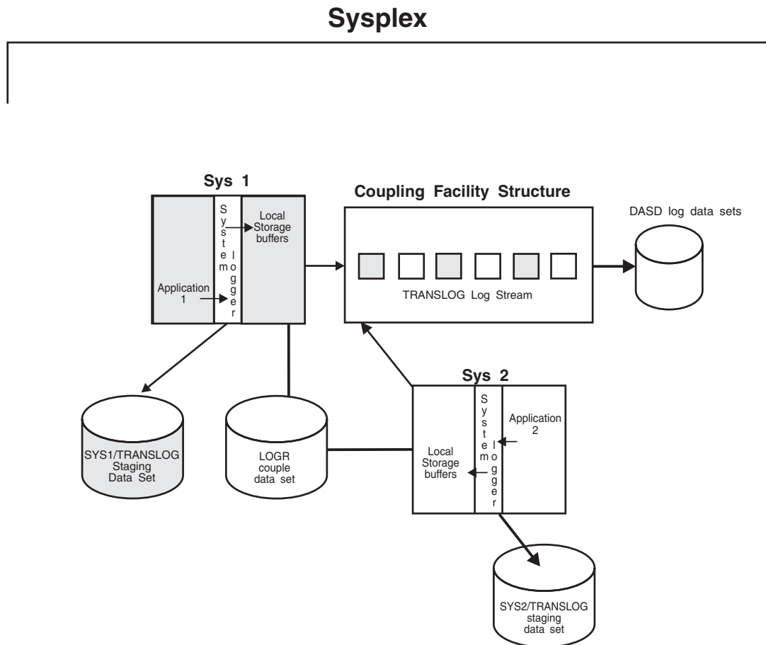
Figure 112. A Complete Coupling Facility Log Stream Configuration
